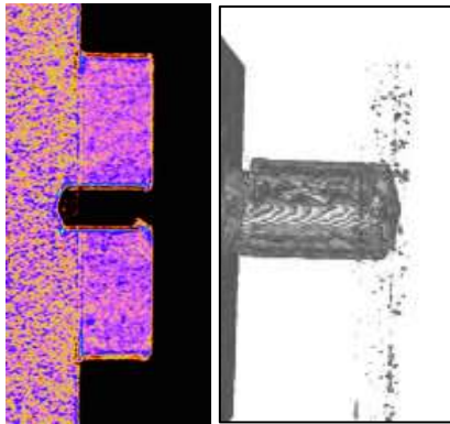
Figure 17 – a) Left - cross-section of a cavity of the Al clip part. b) Right - inverse of the cavity hole.
