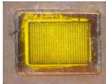
Figure 10 – An optical image of the underside of a mono-mode wave as seen through the PI ablator assembled into bottom of a Vespel clip holder.
