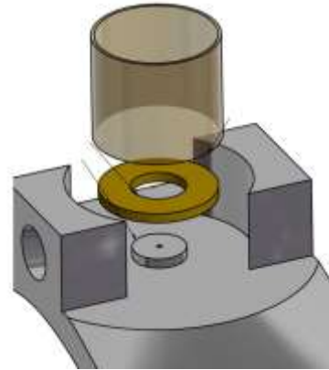
Figure 14 - The Jet launching target design provided by S. Klein (University of Michigan).
