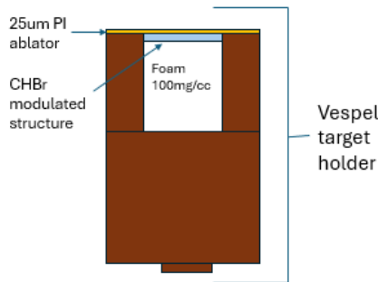
Figure 5 – Basic schematic of the different target design.
