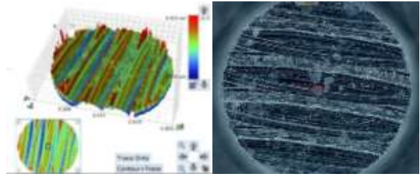
Figure 19 – a) Left - white light interferometry scan showing the very rough surface of the Al part. b) Right - optical image showing the diameter of the cavity and the poor surface quality.
