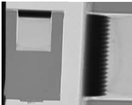
Figure 7 – a) Left - X-ray radiograph checking the foam quality and contact with the modulated interface. b) Right - close-up image showing the poor foam-interface contact.
