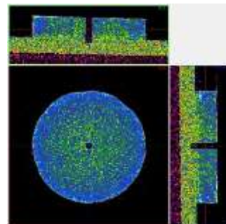
Figure 22 – Example 360-degree X-ray radiography of a straight cavity type within an Al part.
